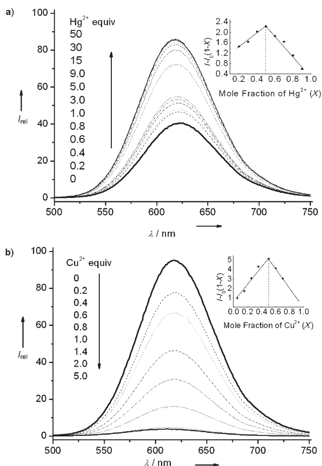
Figure 1. Emission spectra of DCPP (5.0 \mu\text{M} ) in a mixture of \text{H}_2\text{O} and \text{CH}_3\text{CN} (4/6, v/v) with a buffer solution of \text{Na}_2\text{HPO}_4/\text{KH}_2\text{PO}_4 (0.01 M, pH 7.0) upon titrating different molar ratios of \text{Hg}^{2+} (a) and \text{Cu}^{2+} ions (b) with excitation at 440 nm. I_{\text{rel}} = 100 corresponds to I = 1000 in the case of (a) and to I = 390 in the case of (b). Insets: Job's plots; the total concentration of DCPP and \text{Hg}^{2+} or \text{Cu}^{2+} ion is 10.0 \mu\text{M} .
