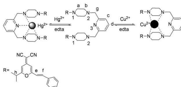
Scheme 2. Proposed sensing process of DCPP by characteristic square-planar coordination with \text{Cu}^{2+} and tetrahedral coordination with \text{Hg}^{2+} , both of which can be reset by addition of edta.
